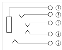
SCHMATIC
